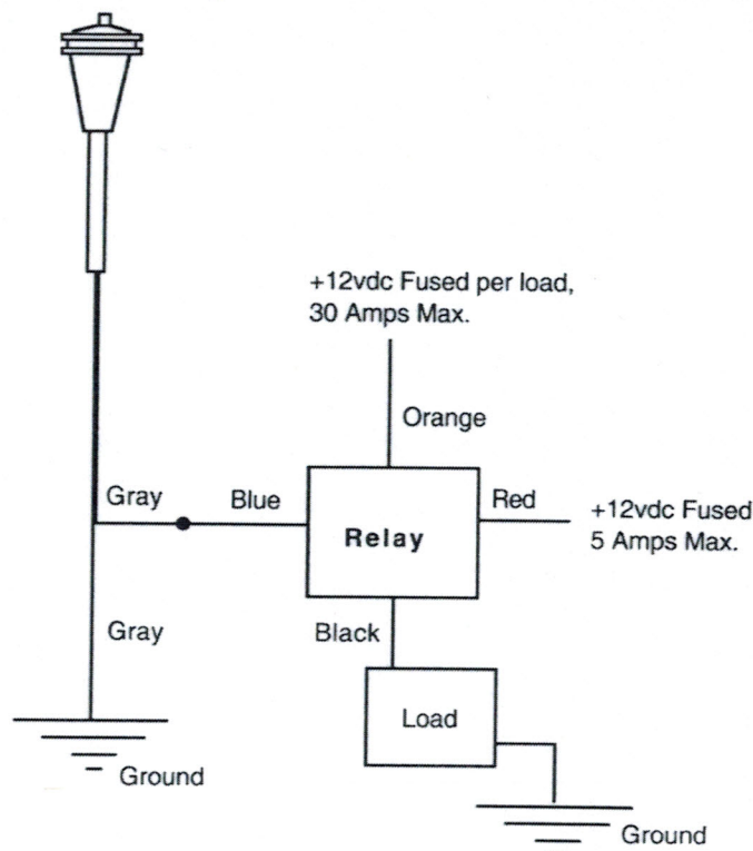
Ground Switching
