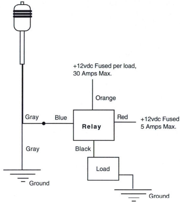
Ground Switching
